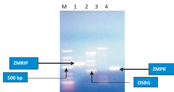
Fig. 58. Amplicons of defense related genes
